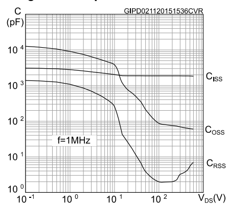
Figure 12: Capacitance variations
