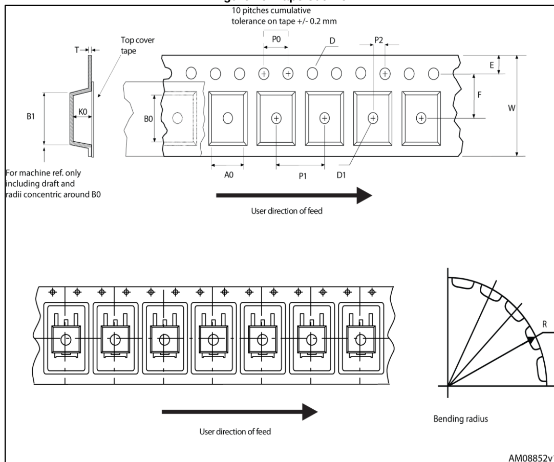
Figure 26: Tape outline
