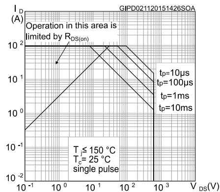
Figure 2: Safe operating area for D 2 PAK
