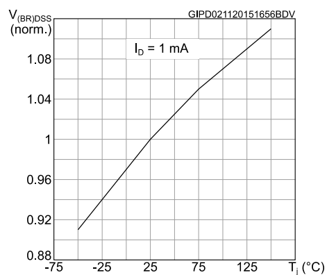
Figure 15: Normalized V_{(BR)DSS} vs temperature
