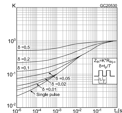
Figure 7: Thermal impedance for TO-247
