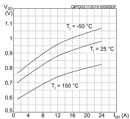
Figure 17: Source-drain diode forward characteristics
